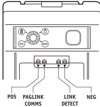
Front Terminals
